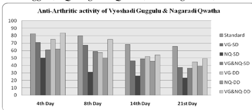
Chart – 1 Anti- Arthritic activities of Vyoshadi Guggulu and Nagaradi Qwatha on Freund's adjuvant induced Arthritis
